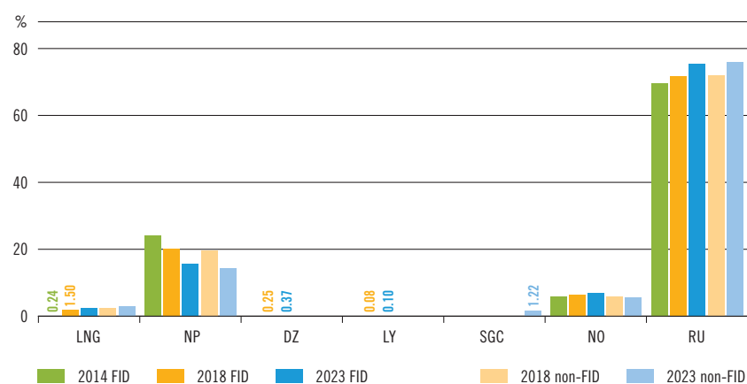
Figure 31: The share of supply sources in the CEE region under maximum deliveries of gas from Algeria and under the average day conditions
