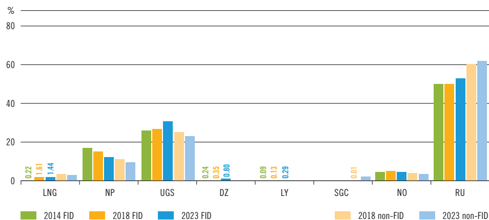
Figure 20: The share of supply sources in the CEE region under the two-week uniform risk day conditions
