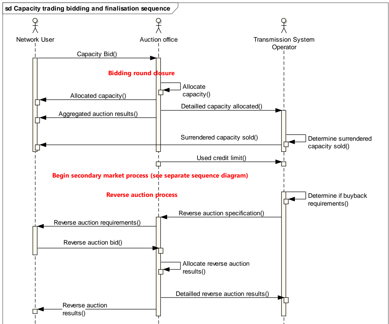
FIGURE 2: SEQUENCE DIAGRAM BIDDING AND FINALISATION OVERVIEW
