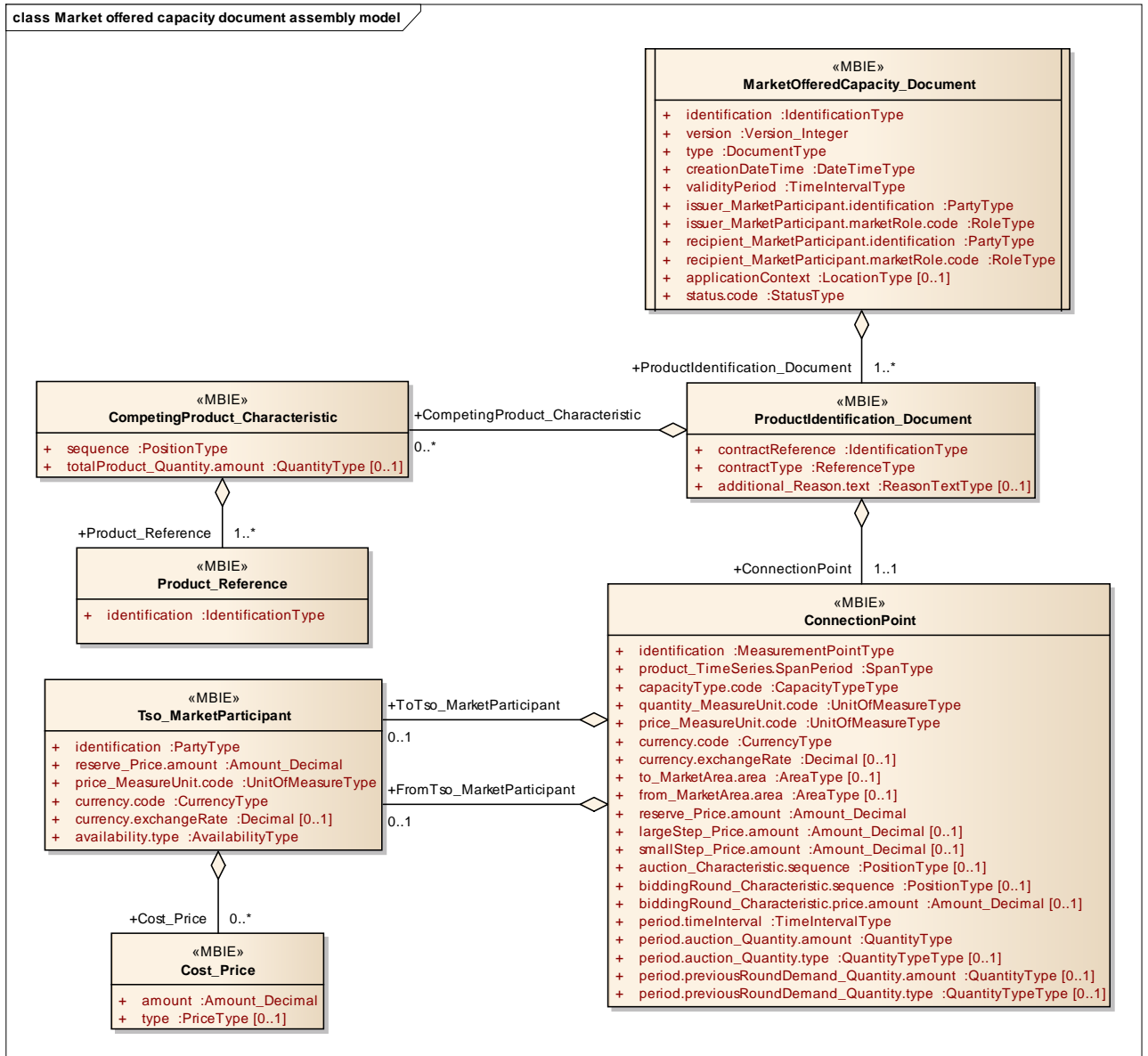
FIGURE 8: MARKET OFFERED CAPACITY DOCUMENT ASSEMBLY MODEL
